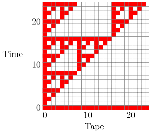
Figure 3: The cellular automaton given by f(x, y) = x \oplus y .
