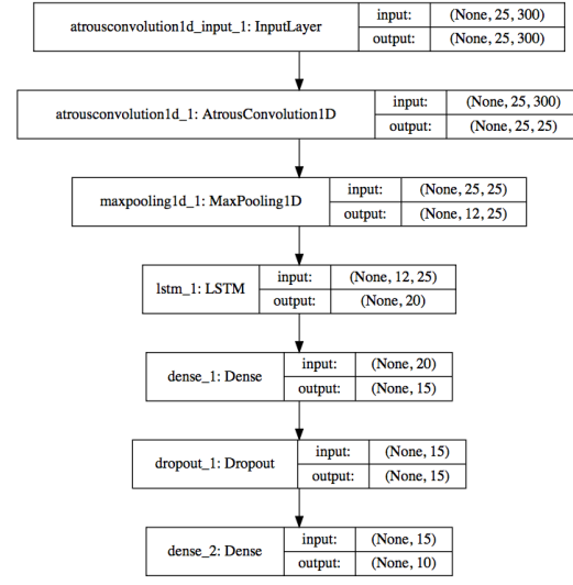
Figure 2: DNN encoder for predicting metaphorical paraphrase aptness from Bizzoni and Lappin (2018) . Each encoder represents a sentence as a 10-dimensional vector. These vectors are concatenated to compute a single score for the pair of input sentences.
