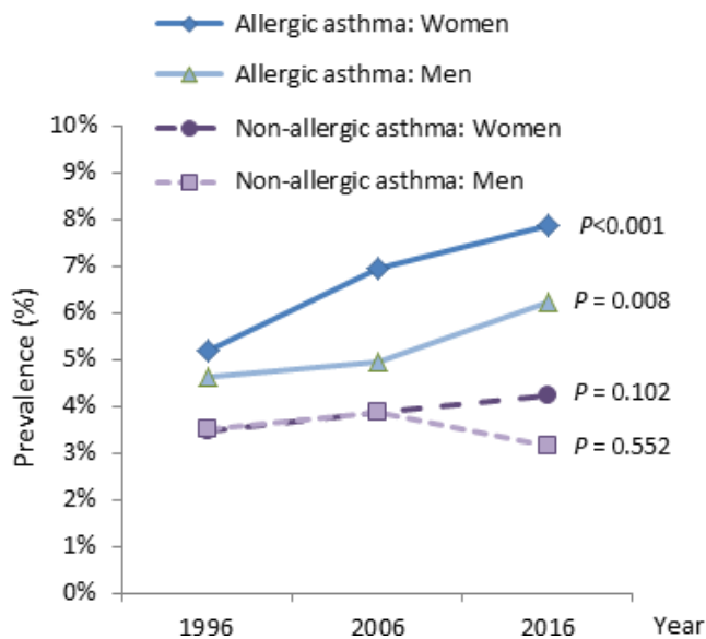
FIGURE 1 Prevalence of allergic and non-allergic asthma, respectively, among men and women. P -value for trend across the 3 y
