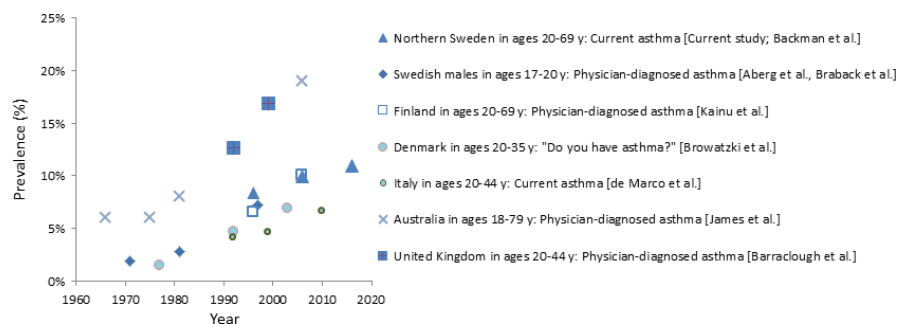
FIGURE 3 Repeated surveys of asthma prevalence among adults in the general population, with the same methods within the same age-span and area
