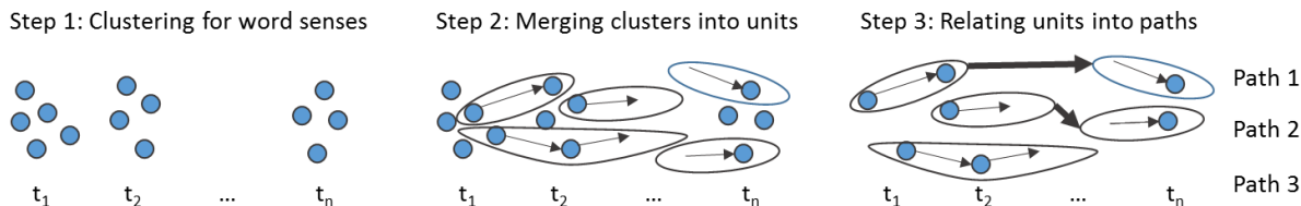
Figure 1: Process for word sense change detection.
