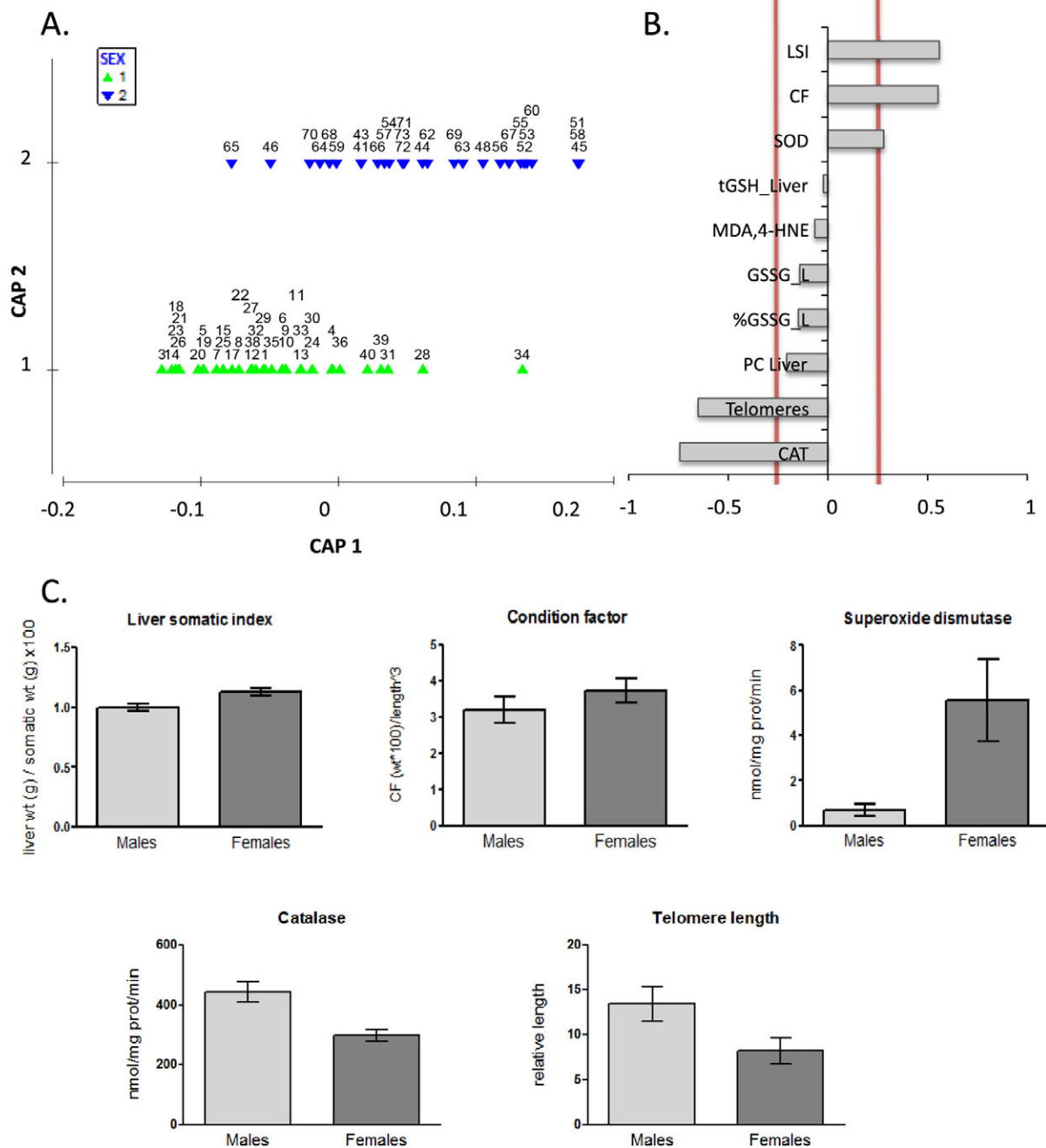
Fig. 1. (A) CAP analysis on sex (1=male, 2=female) for all cod. (B) Correlation analysis for CAP axis 1. Level of significance ( df = 61 ) \pm 0.25 is indicated by red line. Levels of liver somatic index (LSI), condition factor (CF) and superoxide dismutase (SOD) are higher in females, while catalase (CAT) and telomeres are lower, in comparison to males. PERMANOVA, pseudoF 1, 43 =5.6, P=0.001. (C) Results of variables found to differ significantly, illustrating differences between the sexes.
