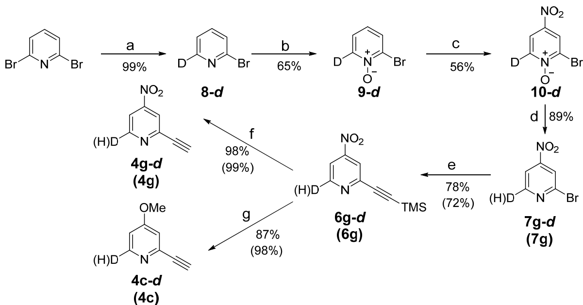
Scheme 3. a Reagents and Conditions: (a) 1. n BuLi (1 equiv.), THF, -78 °C; 2. MeOD (5 equiv.), -78 °C, 1 h, then rt, 24 h; (b) m CPBA, CHCl 3 , rt, 24 h; (c) HNO 3 /H 2 SO 4 2:1, 110 °C, 3 h; (d) PBr 3 , CH 2 Cl 2 , 60 °C, 3 h; (e) TMS-acetylene, Pd(PPh 3 ) 2 Cl 2 , CuI, Et 3 N, 5 °C, 1 h, then rt, 2 h; (f) KF, MeOH, rt, 2 h; (g) K 2 CO 3 , THF/MeOH 1:1, rt, 1 h.
