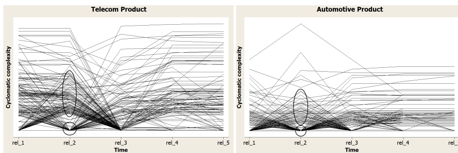
Figure 1: Evolution of M of functions
