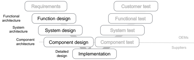
Fig. 1. V-model with the focus on architectural views and evolution.
