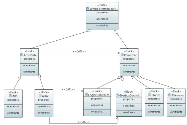
Fig. 4. Example of a logical view – a UML class diagram notation.
