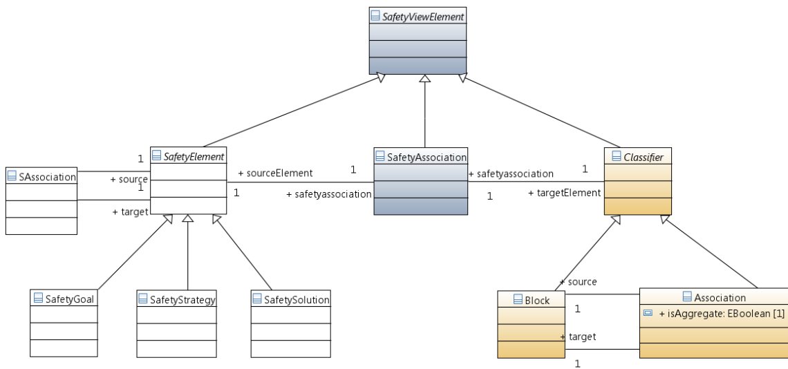
Fig. 5. The meta-model of the safety view.
