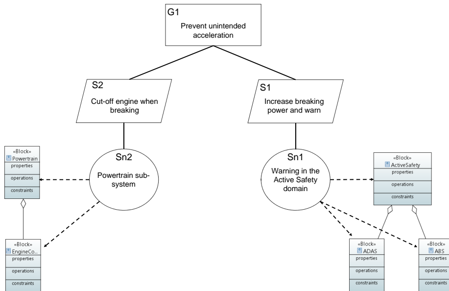
Fig. 6. Example of a safety view combining two notations.
