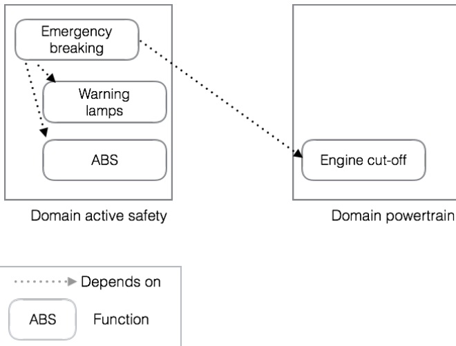
Fig. 2. Example of a functional architecture – or a functional view.
