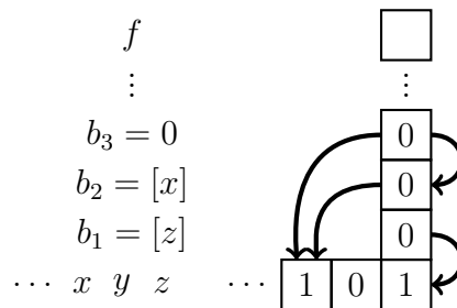
Figure 7: A modular game \mathcal{G}'' whose output function f is identical to that of \mathcal{G}' . The only difference is that \mathcal{G}'' does not check for the pattern 101. The box b_3 contains a 0 independently of the input xyz to f .
