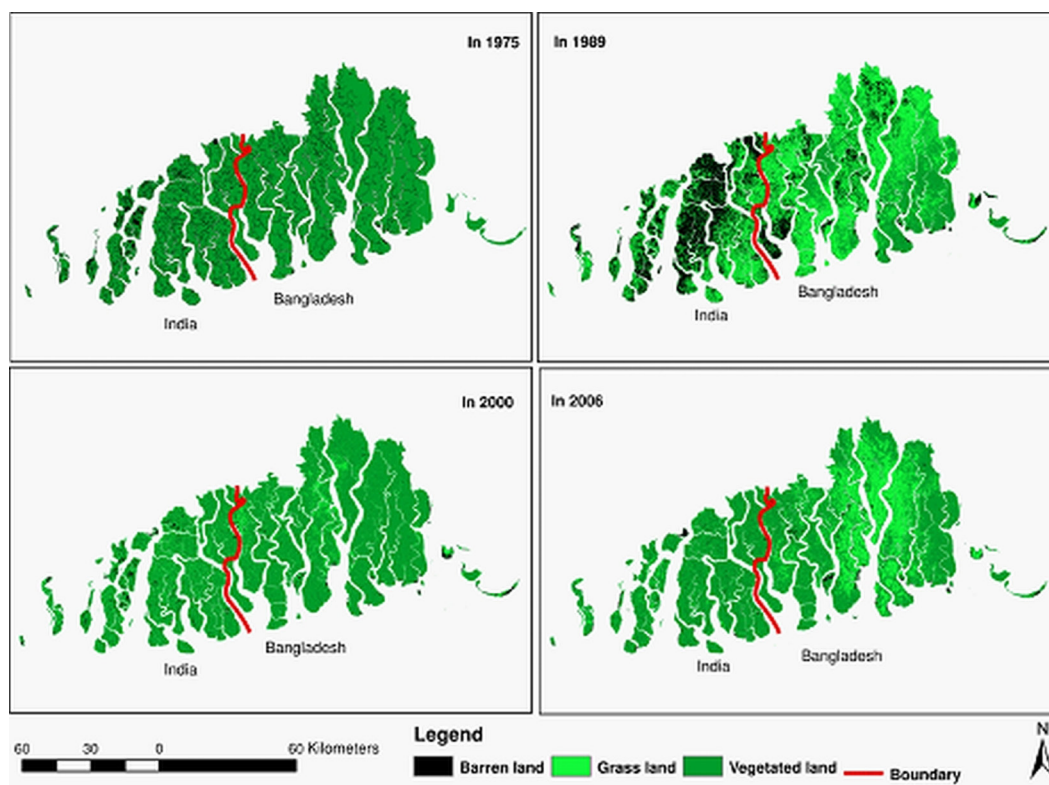
Fig. 4. Land covers in Sundarbans except water channels
