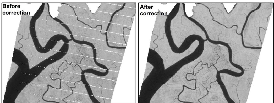
Fig. 2. A section of image D1
