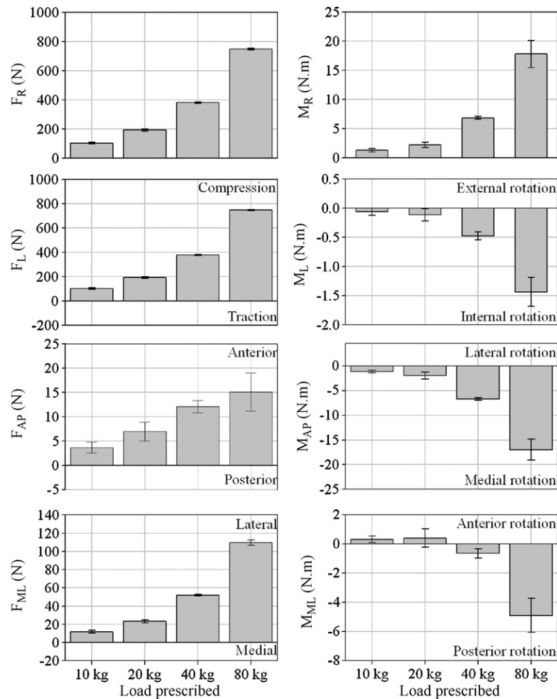
Fig. 2. Overall mean and one standard deviation of forces ( F ) and moments ( M ) applied on and around medio-lateral (ML), antero-posterior (AP) and long ( L ) axes, and the resultant ( R ) for the three trials in each load prescribed.
