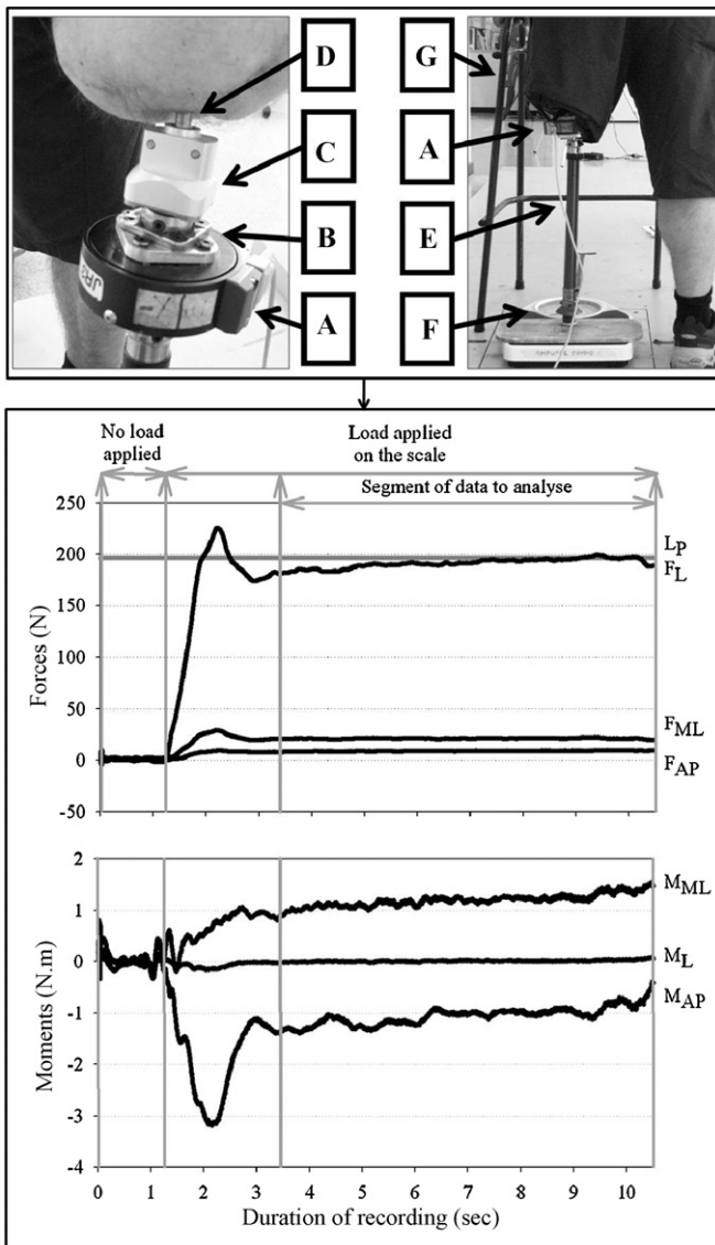
Fig. 1. Measurement of loading including a six-channel transducer (A), mounted between plates (B), connected to an adaptor (C), the abutment of the osseointegrated fixation (D) and a long pylon (E), a frame (G), and a weighing scale (F). Example of loading profile and segment of data to analyse for forces (F) and moments (M) applied on and around the medio-lateral (ML), antero-posterior (AP) and long (L) axes of the abutment when the load prescribed ( L_p ) applied on the scale was 20 kg (196.20 N).
