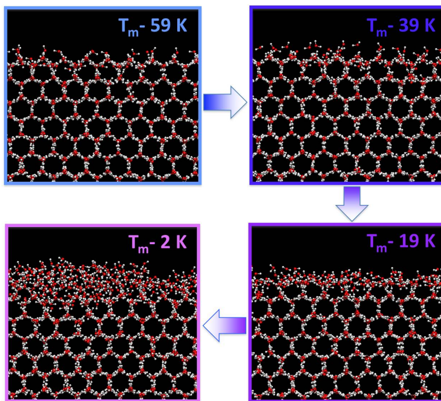
Fig. 8. Snapshots of the prismatic air–ice interface for selected simulations. The simulation temperatures correspond to undercooling of -59\text{ K} through -2\text{ K} relative to the melting point of the water model (NE6, T_m = 289\text{ K} ). Reproduced from Gladich et al. (2011) with permission from the PCCP Owner Societies.
