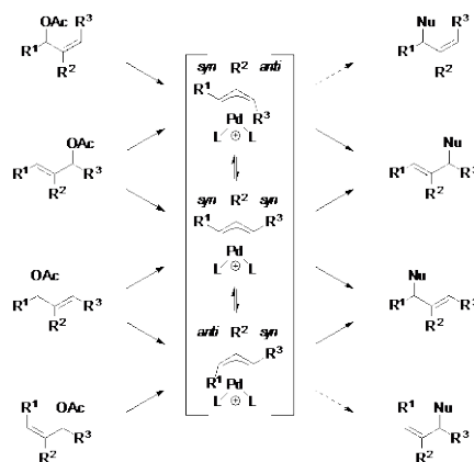
Scheme 1. The Dynamic Manifold of Intermediates in Pd-Assisted Allylic Alkylation
