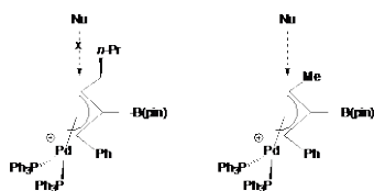
Figure 1. Interference between alkyl group and incoming nucleophile.
