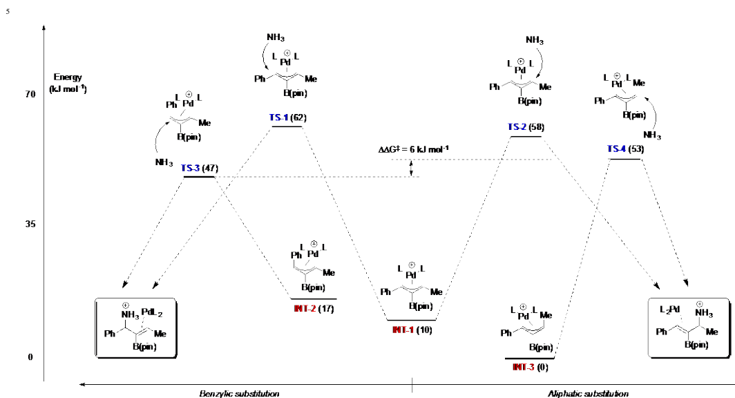
Figure 3. Calculated energy diagram for allylic substitution leading to benzylic and aliphatic substitution products. Values in parentheses are the energies relative to 1- syn , 3- anti INT-3.
